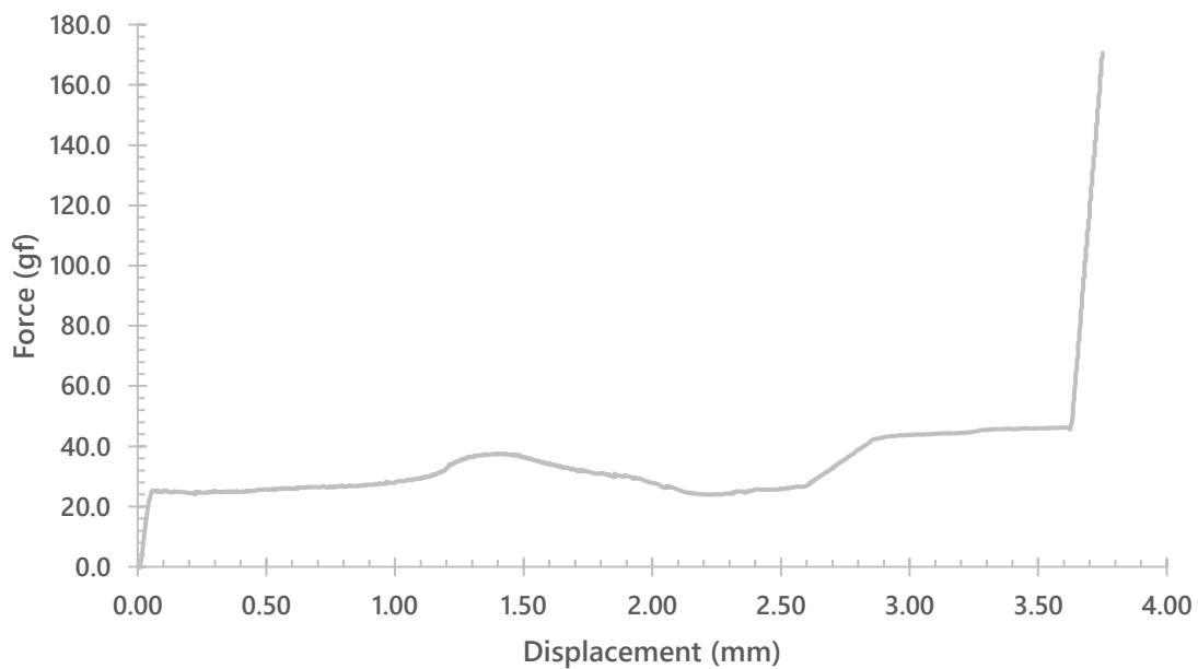
Gateron Chocolate Jelly (Upstroke)
